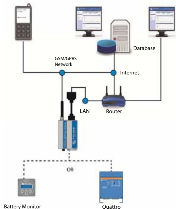
Victron Ethernet Remote
